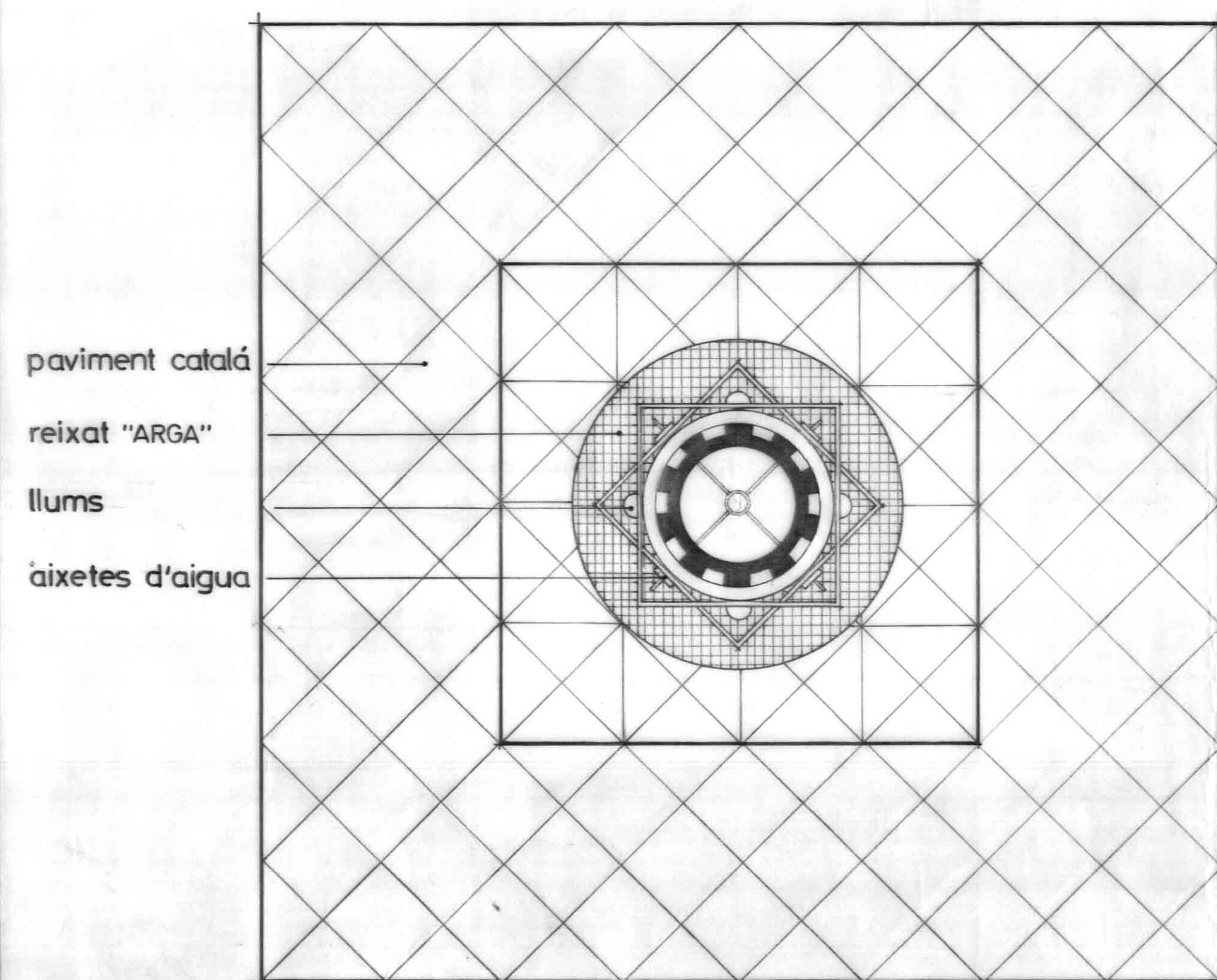
PLANTA E: 1/20 modul ortogonal: 50 cms.
